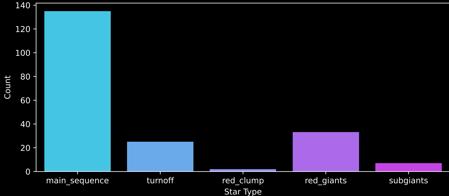
APOGEE DR17 Field: [K2_C14_230+55] Count plot of Star Type
