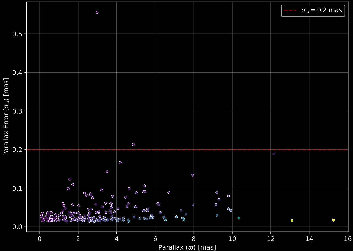
APOGEE DR17 Field: [K2_C14_230+55] Parallax Quality (n= 202)
