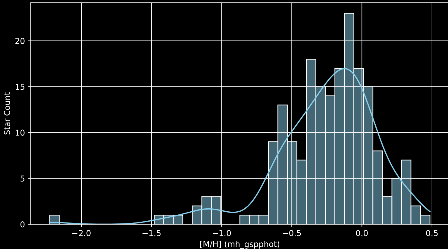
APOGEE DR17 Field: [K2_C14_230+55 [M/H] (mh_gspphot) (n= 198)
