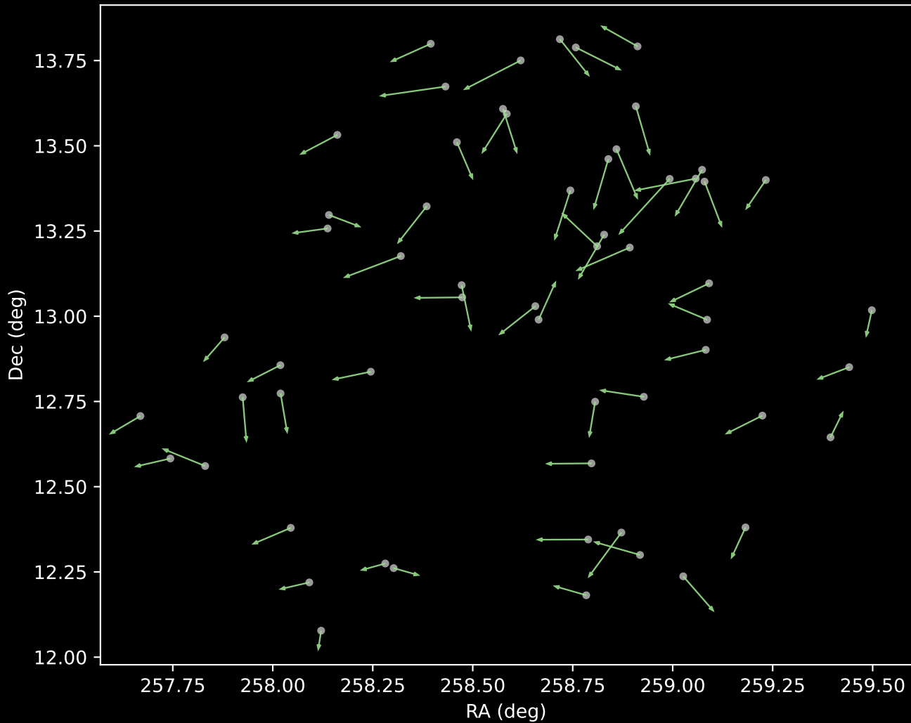
APOGEE DR17 Cluster 5 Proper Motion Vectors (n=59)
