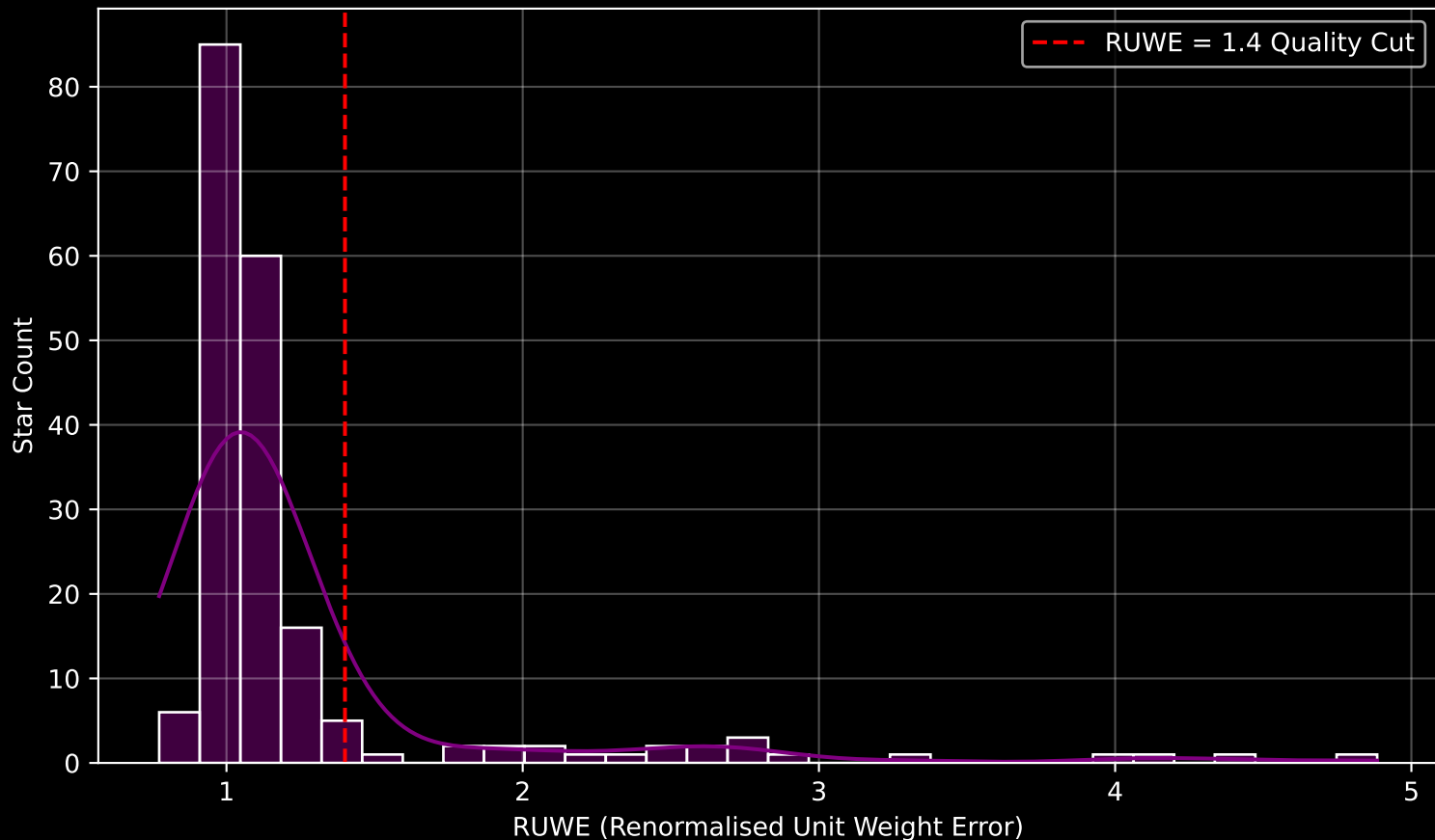
GAPOGEE DR17 Field [K2_C14_230+55] RUWE Distribution (n= 194)
