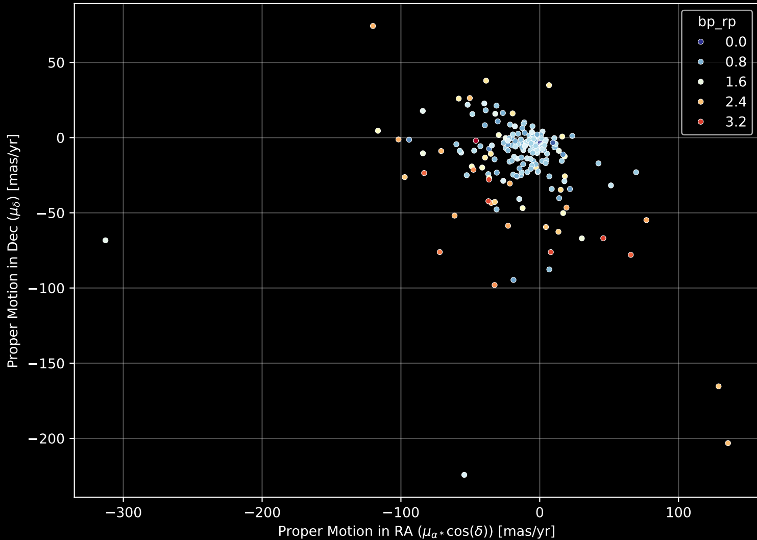
APOGEE DR17 Field: [K2_C14_230+55] Proper Motion Diagram (n= 202)
