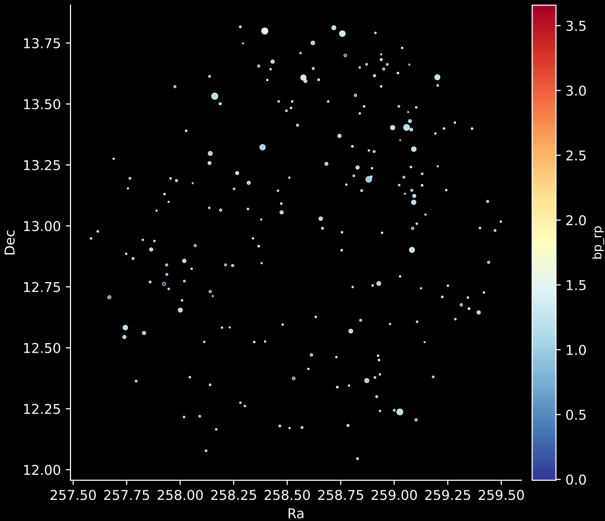
APOGEE DR17 Field: [K2_C14_230+55] Stars: 202
